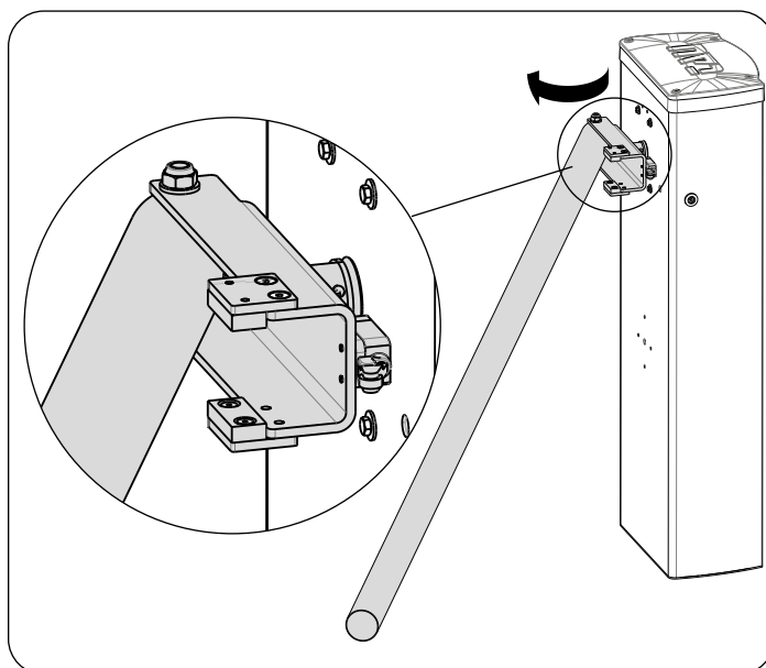
Breakout system for round boom (800SFA)
